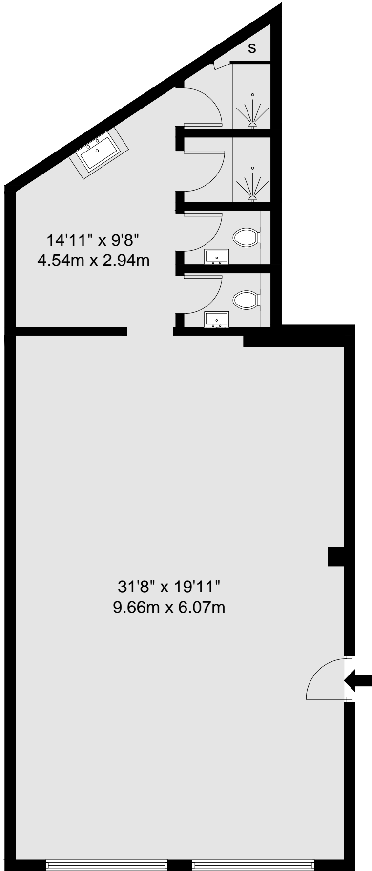
Ground Floor
