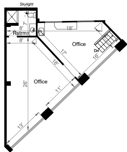
SECOND FLOOR 775 SQ FT
