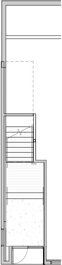
1 FIRST FLOOR PLAN 33-B A-4/4 1" = 10'-0"
