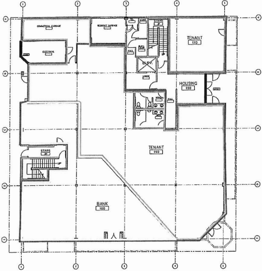
1st FLOOR PLAN NTS
