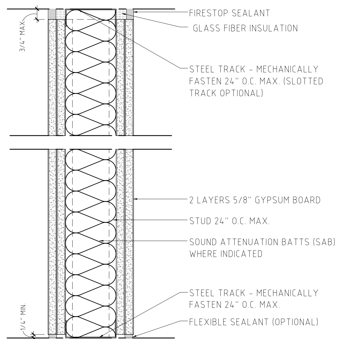
2 PARTITION TYPE 3" = 1'-0" ONE-HOUR FIRE RATED - UL LISTING: U411
